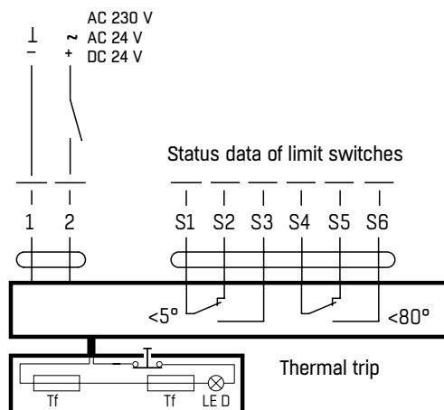
Fig. 2. Wiring diagram for damper motor
