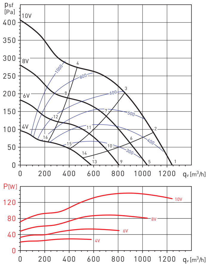
TD-1300/250 SILENT ECOWATT
