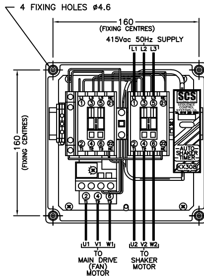
FRONT COVER REMOVED TO SHOW FIXING HOLES & EXTERNAL CONNECTIONS
